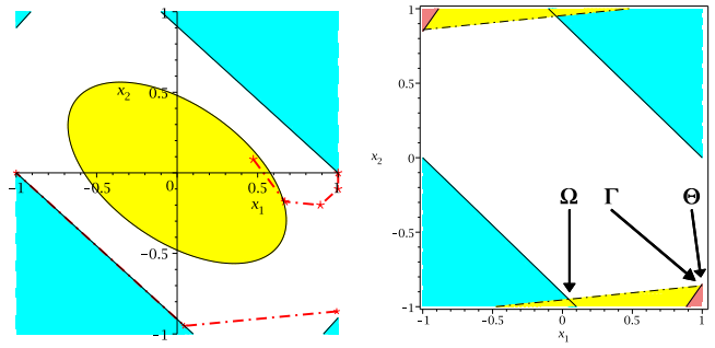
Fig. 1. (left): Representation of two trajectories (dotted curves in red) for the system with control u = 1 at each step, starting at (1, 0) and \Gamma . The feasible set \mathcal{F}_1 in white, \mathcal{N} in yellow (oval shaped). (right): The constraints defining \mathcal{F}_1 (blue) and \mathcal{F}_2 (yellow) intersect in \Omega (on the half space x_2 \leq 0 ). Analogously \Gamma is defined as intersection of \mathcal{F}_2 and \mathcal{F}_3 (red, \mathcal{F}_3 = \mathcal{F}_\infty ). \Theta is the intersection with the line x_1 = 1 .
