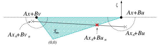
Fig. 3. Continuity proof in \mathbb{R}^2 , Theorem 17(iii).
